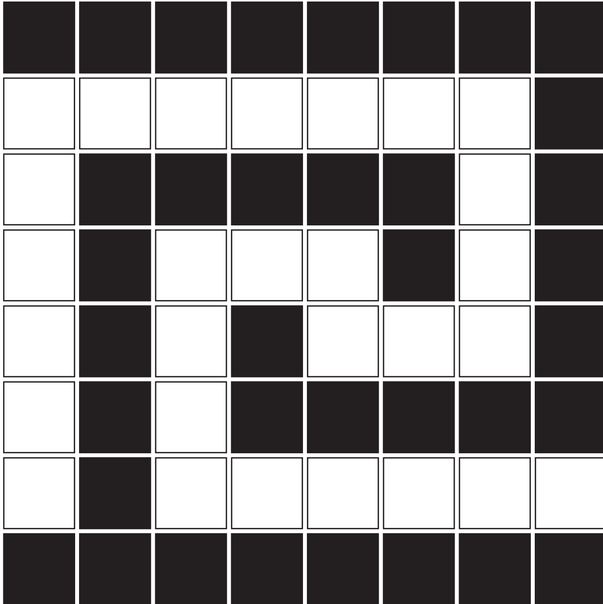
3/4" Tile Template
